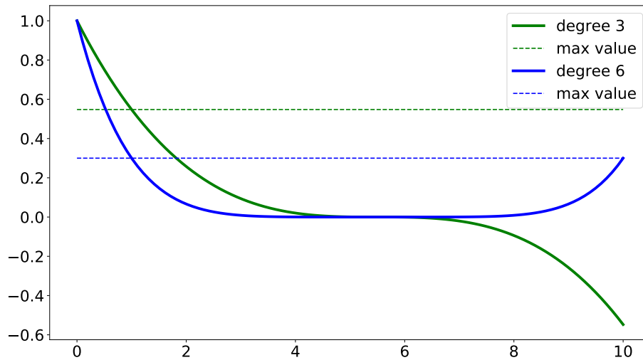
Figure 1: Naive Polynomial
